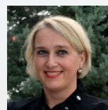
A.M. Simundic
